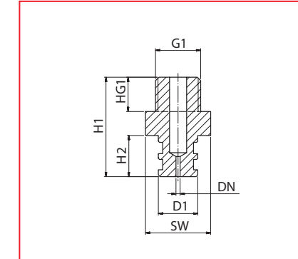
ANF-8-M5, ANF-8-1/4
