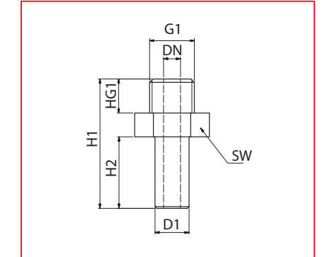
ANF-10-1/4, ANF-16-1/4
