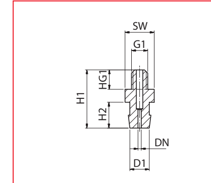
ANF-6-M5, ANF-6-1/4
