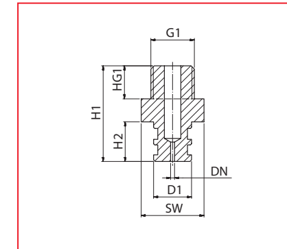
ANM-8-1/8, ANM-13-1/4
