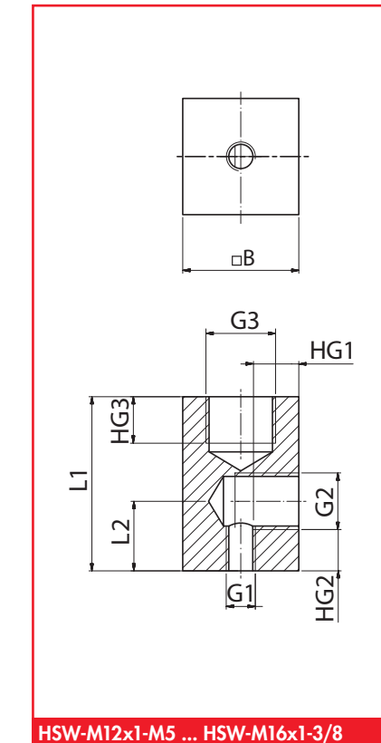
HSW-M12x1-M5 ... HSW-M16x1-3/8
