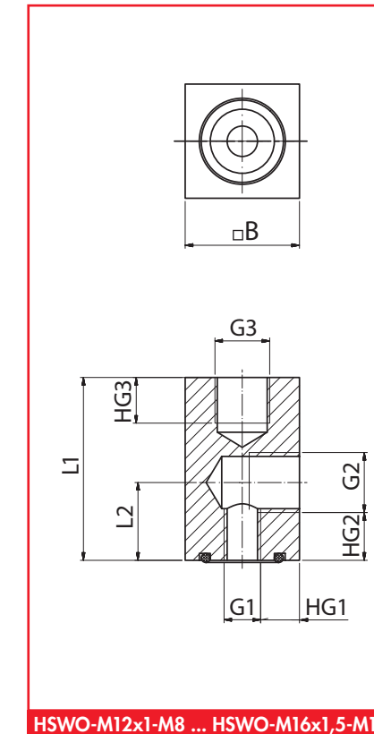
HSWO-M12x1-M8 ... HSWO-M16x1,5-M16
